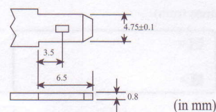
Optional Terminal B1-(copper) Bolt Type: M5
