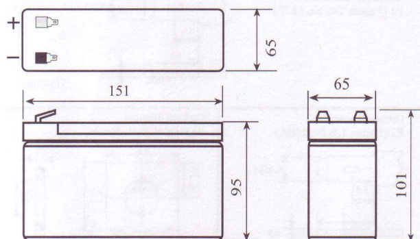
Dimensions (mm)
