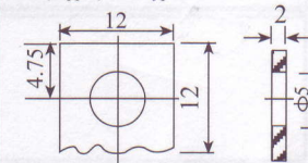
Optional Terminal B1-(copper) Bolt Type: M5
